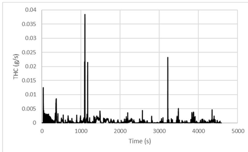
Figure 33: Mass Rate (g/s) of THC Emissions for Propane School Bus from Cold Morgantown Route
